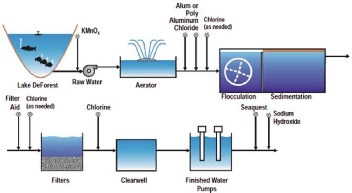
Fig.Flowchart of water treatment plant
